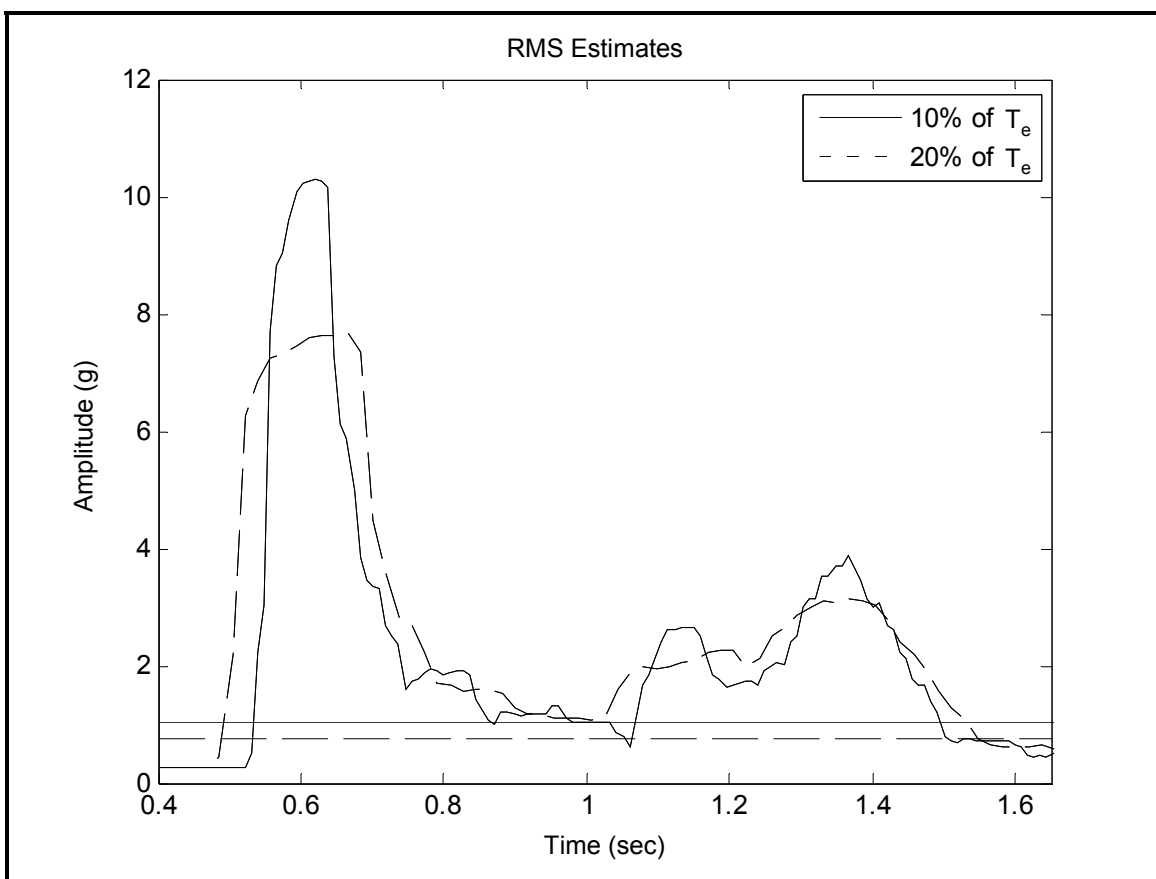
Figure 516.6-4. Response acceleration short-time root-mean-square with averaging time of 10% and 20% of T_e .
