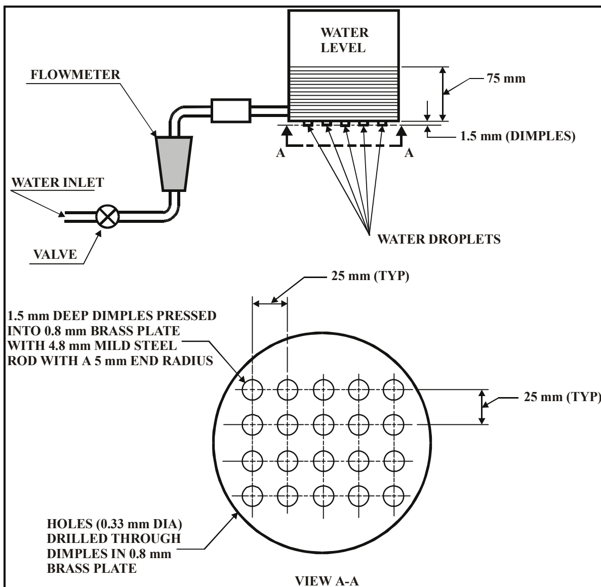
Figure 506.5-3. Details of dispenser for drip test, Procedure III.
