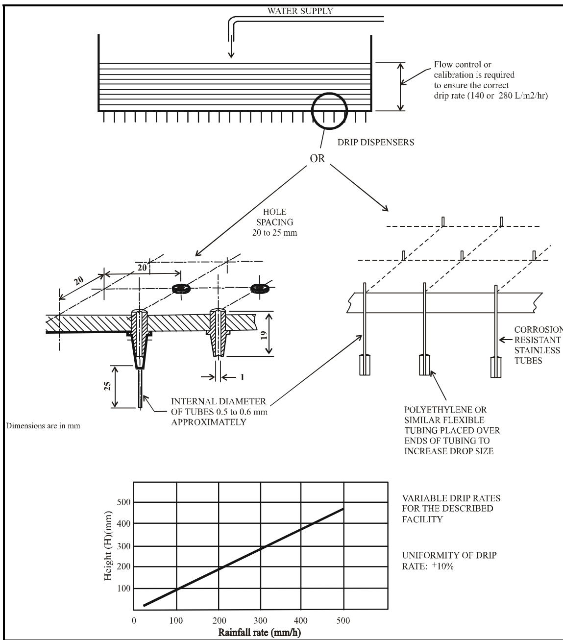
Figure 506.5-1. Sample facility for steady state rain or drip test.
